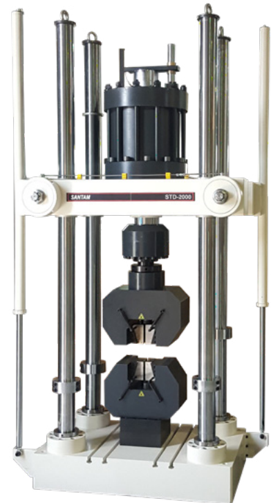
STD-2000 with Hydraulic Wedge Grips
