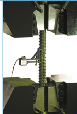
EHR10 Clip-on extensometer Gauge-25 High Resolution 10 mm Travel
