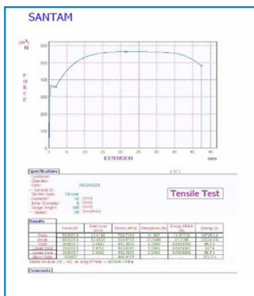
Tensile test Reporting Through Extensometer
