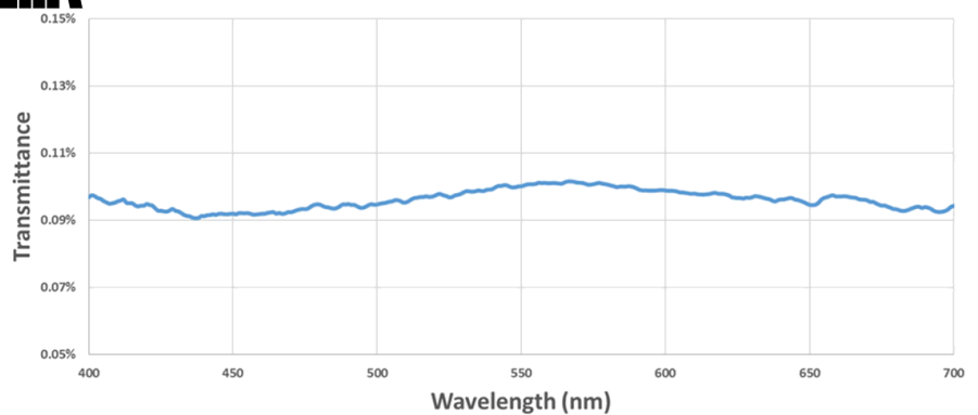
ND1024C Transmission
